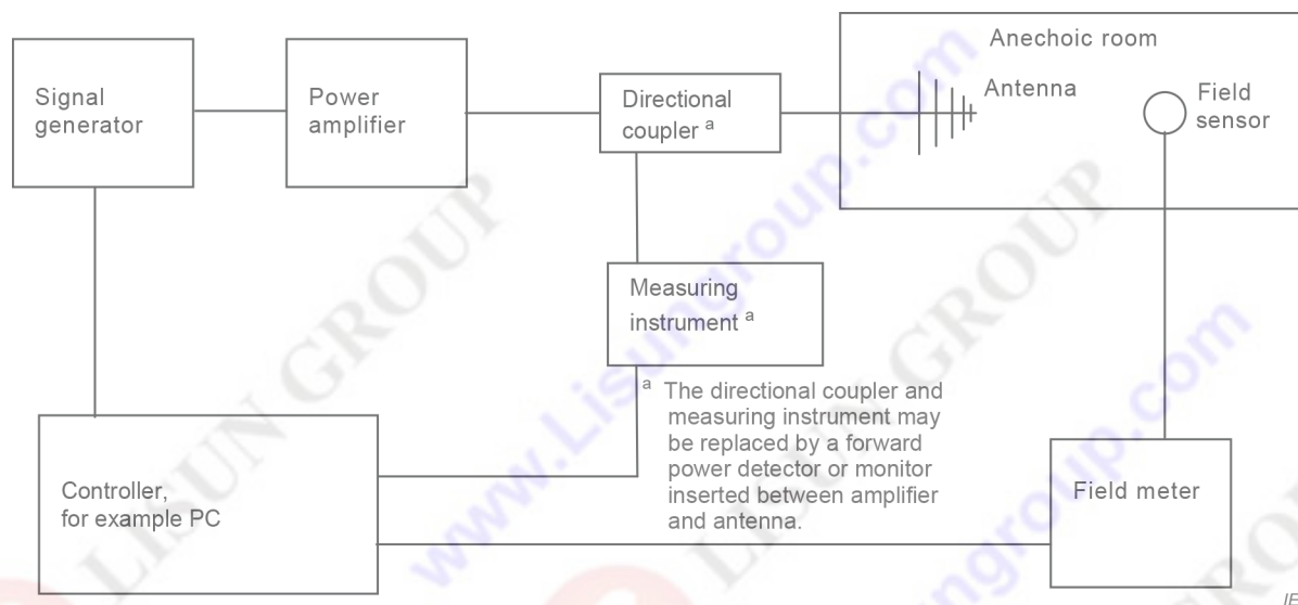
Figure 6 – Measuring setup
