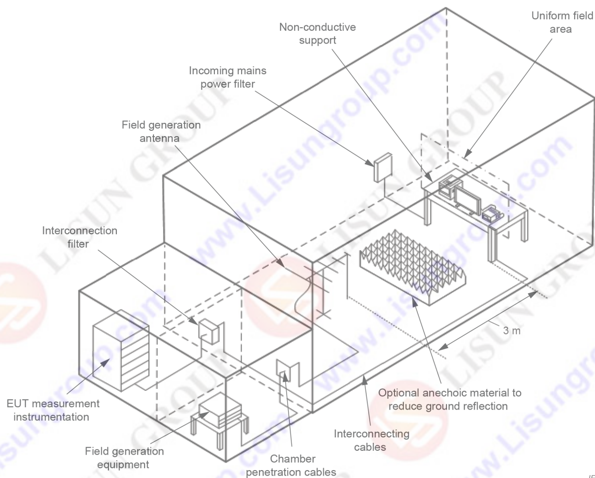
Figure 2 – Example of suitable test facility
