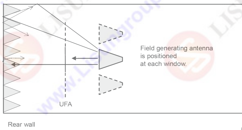
Figure C.2 – Most of the reflected waves are eliminated (applies for top and side view)
