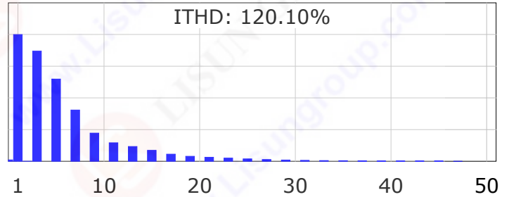
Current Spectrum
