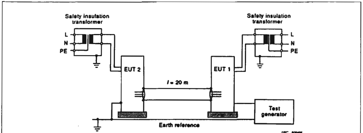
Figure 13 — Example of test set-up for tests applied to shielded lines (according to 7.5) and to apply potential differences (according to 7.6), conductive coupling
