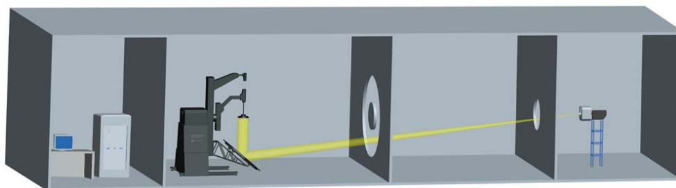
Full View for LSG-5000CCD Moving Detector Goniospectroradiometer
