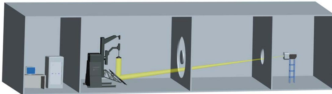
Fig: LSG-5000CCD lab dark room view
