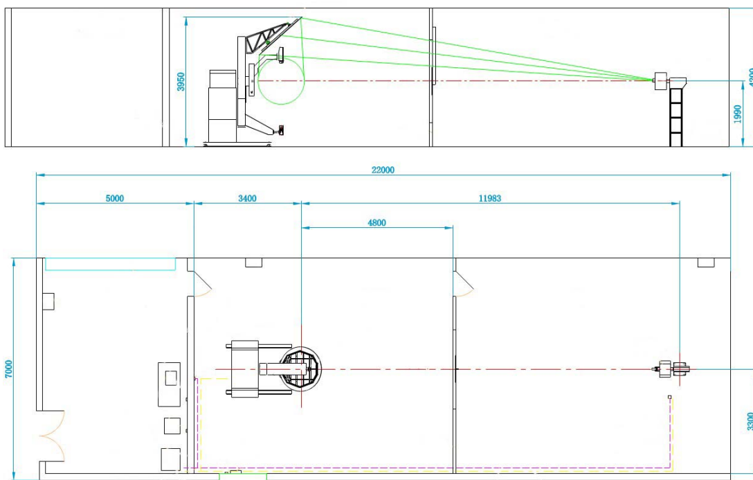
Fig: LSG-5000CCD lab dark room view
